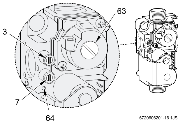
Fig. 17 Valvola gas
